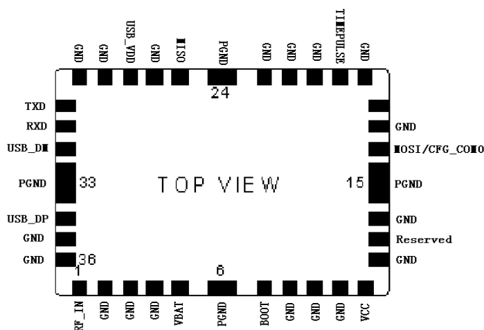
Figure 2: GT-1613-UB Pin Packag
