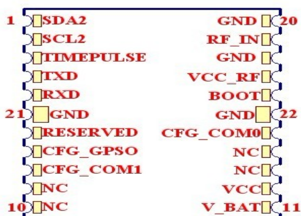
Figure 2: GT-1513-UB Pin Packag
