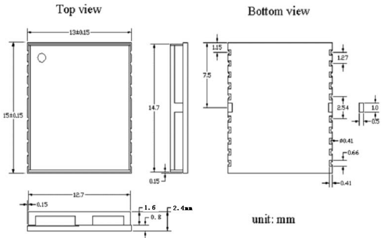
Figure 3: GT-1513-UB Dimensions
