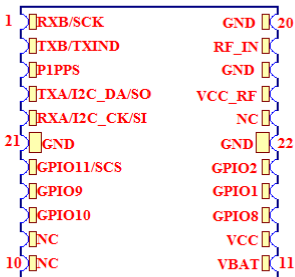
Figure 2: GT-1513-MT Pin Package
