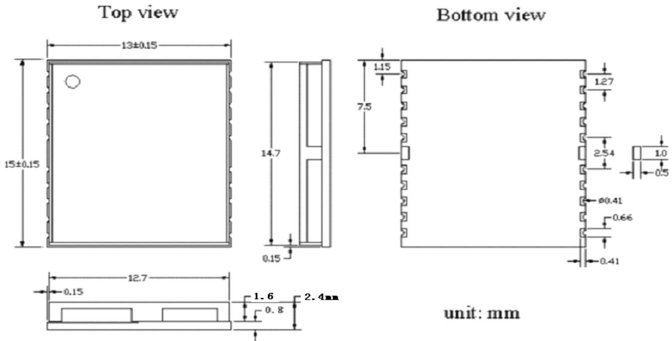
Figure 3: GT-1513-MT Dimensions
