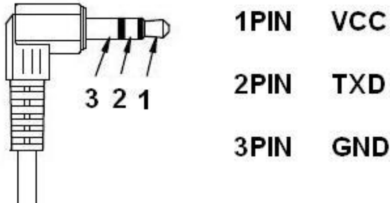
Figure 2: OD3.5 DC Connrctor TopView
